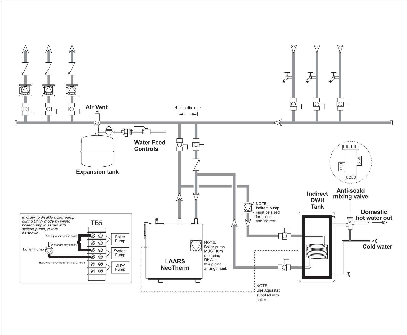
Figure 19. Hydronic Piping — Heating zones with indirect DWH tank piped with zone pumps (indirect directly off boiler). Boiler pump must shut down during DHW.
